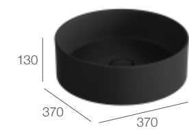
370x370x130 mm S30CB015-02 | Ceramic Waste for Basin
