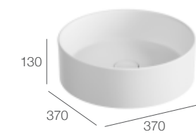
370x370x130 mm S30CB015-01 | Ceramic Waste for Basin
